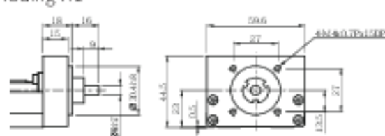
Motor Housing H1
