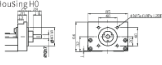
Motor Housing H0
